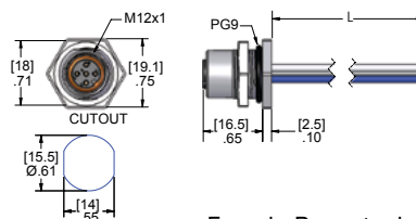
Female Receptacle
