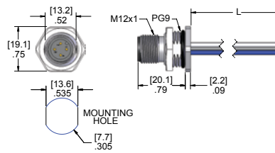
Male Receptacle
