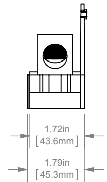
BACK VIEW ADDER (MPDB67000) SHOWN
