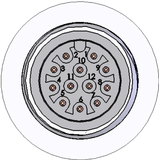
DETAIL A SCALE 5 : 1
