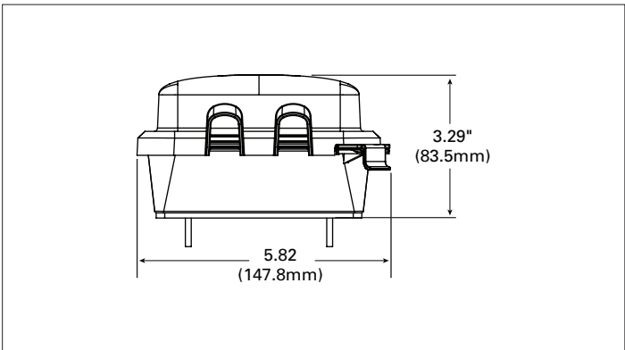
Figure 4. WIU-1HX Horizontal 1-Gang
