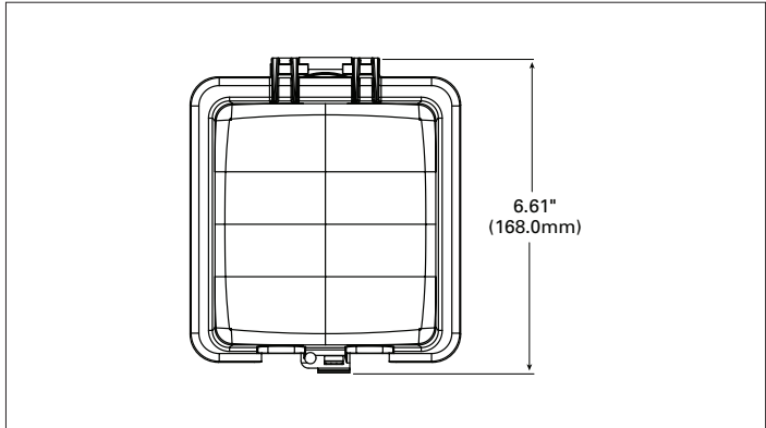
Figure 5. WIU-2X Horizontal/Vertical 2-Gang
