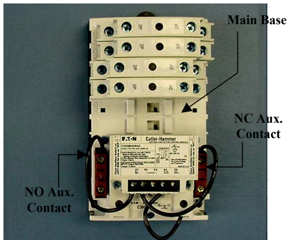
Figure 1: Mechanically Held Contactor
