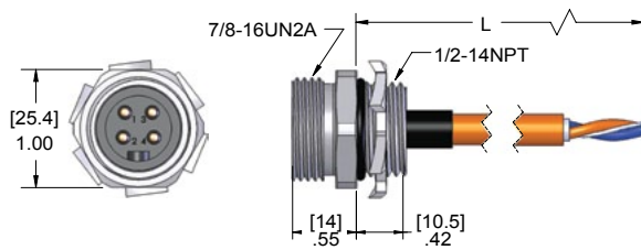
Male Receptacle
