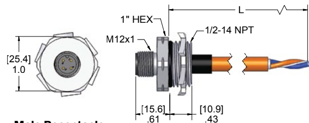
Male Receptacle
