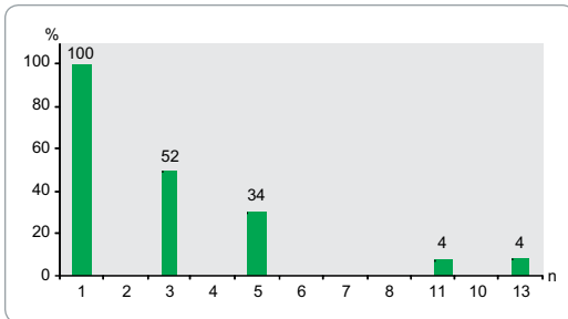
Fig. 16 Harmonic spectrum for single phase industrial devices, induction furnaces, welding machines, rectifiers, etc.
