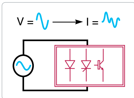
Fig. 19 Non-linear loads are those that generate harmonics.
