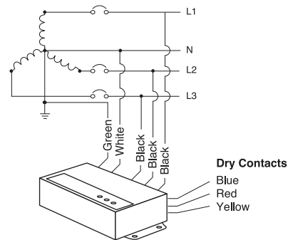
Figure 7: Three-Phase, three- or four-Wire, High-Leg Delta Installation
