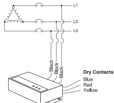
Figure 8: Three-Phase, three-Wire, Delta Installation
