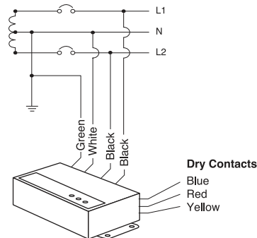
Figure 6: Three-Phase, three- or four-Wire, Grounded Wye Installation
