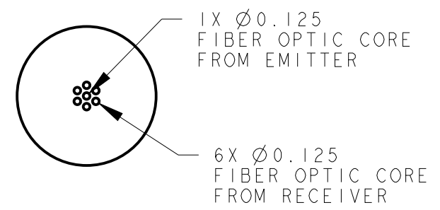
DETAIL A SCALE 10:1
