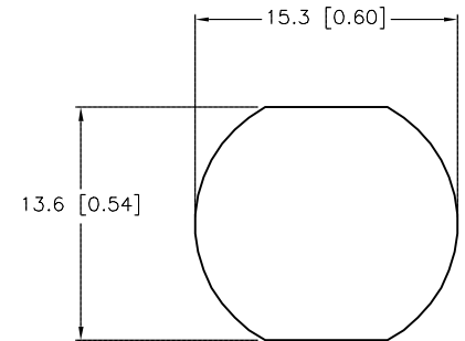
TYPICAL PANEL CUTOUT
