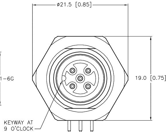
END VIEW
