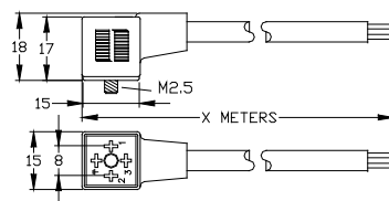
3 Poles + Ground (Ground Opposite Cable Side)
