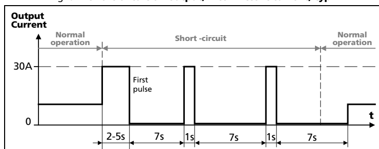
Fig. 6-2 Short-circuit on output, intermittent current, typ.
