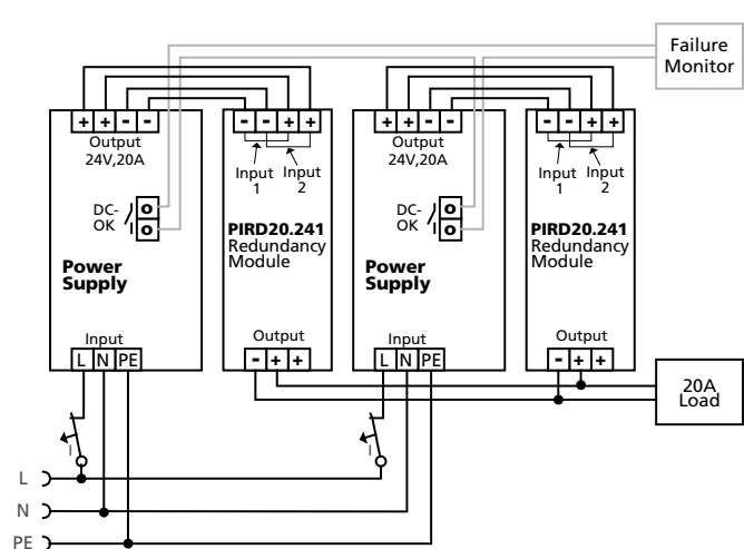
Fig. 23-2 1+1 Redundant wiring with 2 PIRD20.241
