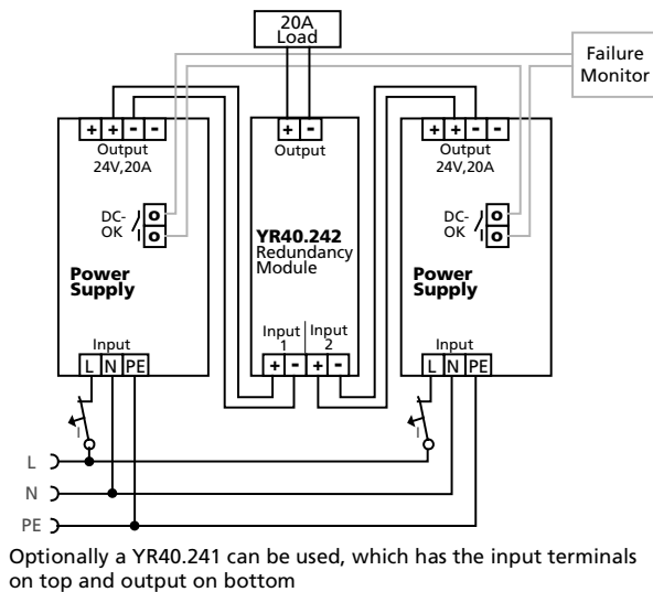
Fig. 23-1 1+1 Redundant wiring with 1 YR40.242
