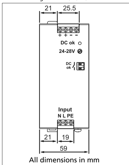
Fig. 21-1 Front view
