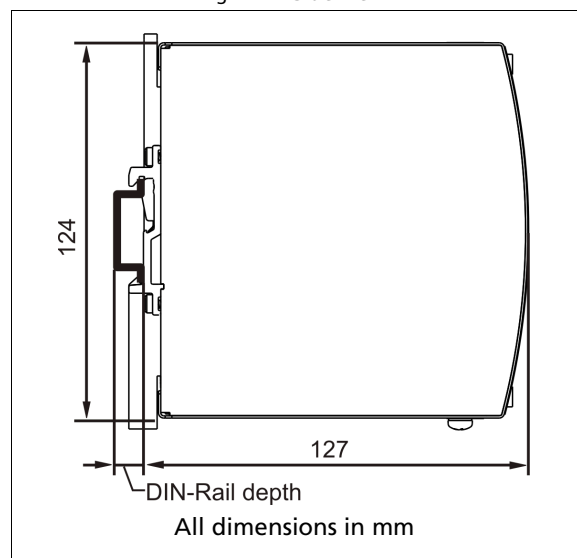
Fig. 21-2 Side view
