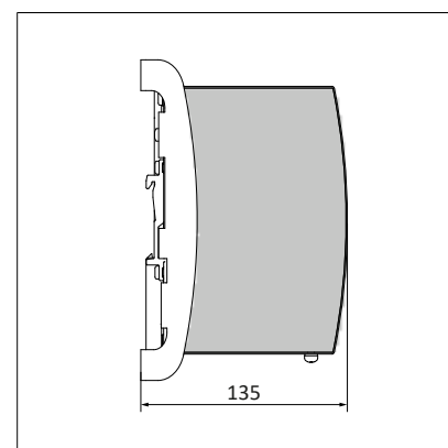
Fig. 23-6: Wall/panel mounting, side view
