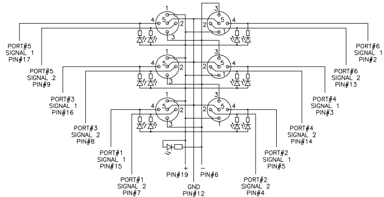
WIRING DIAGRAM
