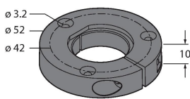
RA2-QR24 1590929 Adapter sleeve, for Ø 14 mm shafts
