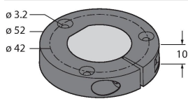
PE1-QR24 1590937 Positioning element without adapter sleeve
