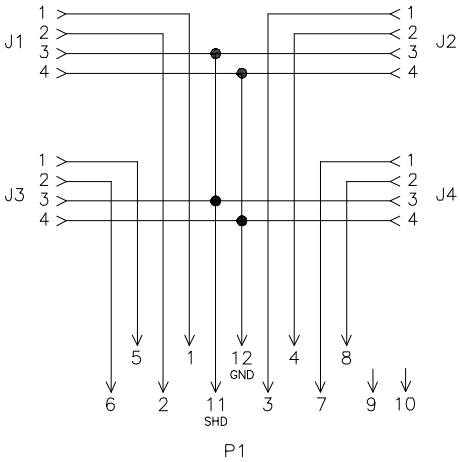
WIRING DIAGRAM
