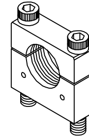
ISOMETRIC VIEW HALF SCALE
