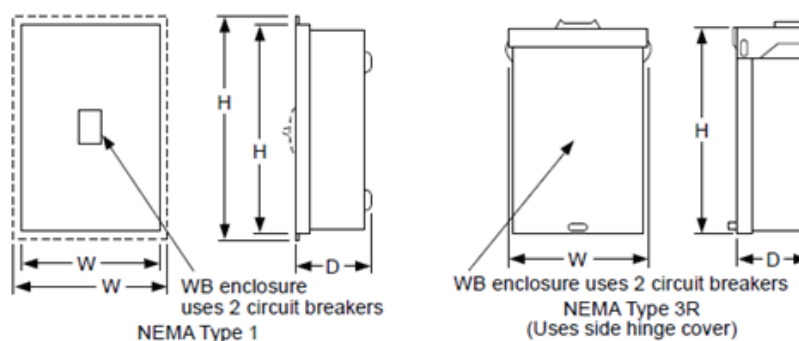
Figure 4 - Enclosure Dimensions
