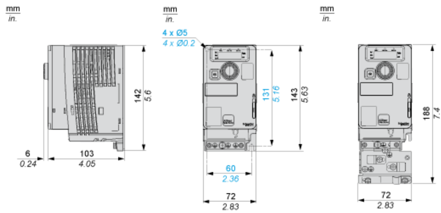
Right View, Front View and Front View with EMC Plate
