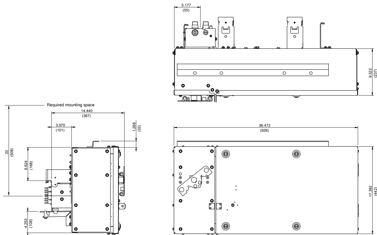
Figure 123 - Circuit Breaker Plug-In Units — 250–600 A
