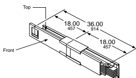
Figure 44 - Unfused Reducer Dimensions
