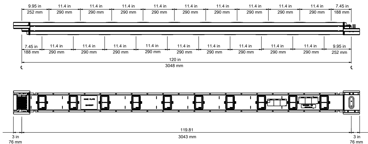
Figure 137 - Ten-Foot Straight Lengths—Enhanced Plug-In Offer
