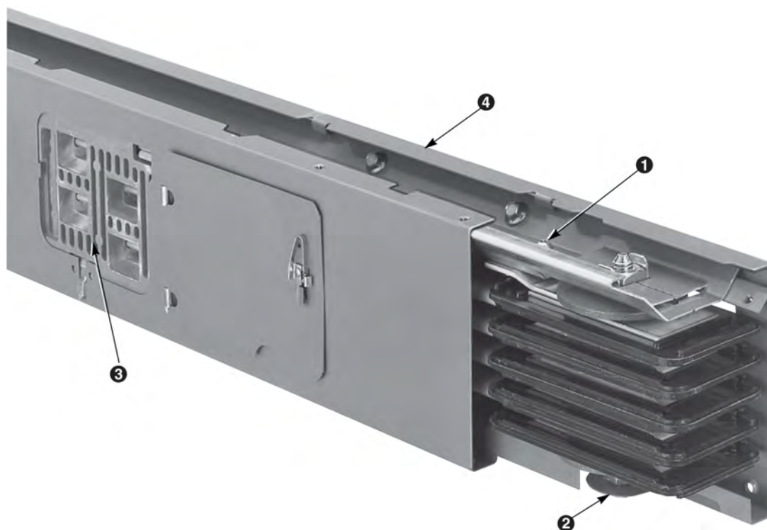
Figure 7 - Plug-In Busway 225–600 A
