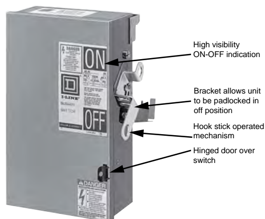
Figure 109 - Fusible Unit
