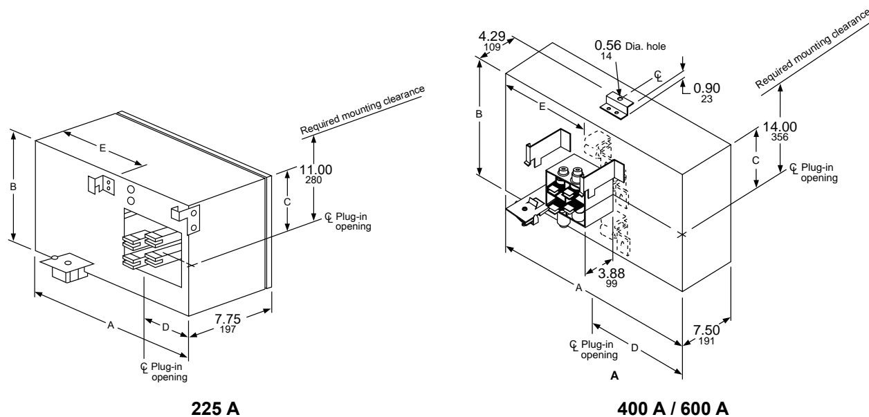
Figure 36 - Cable Tap Boxes (Plug-In)
