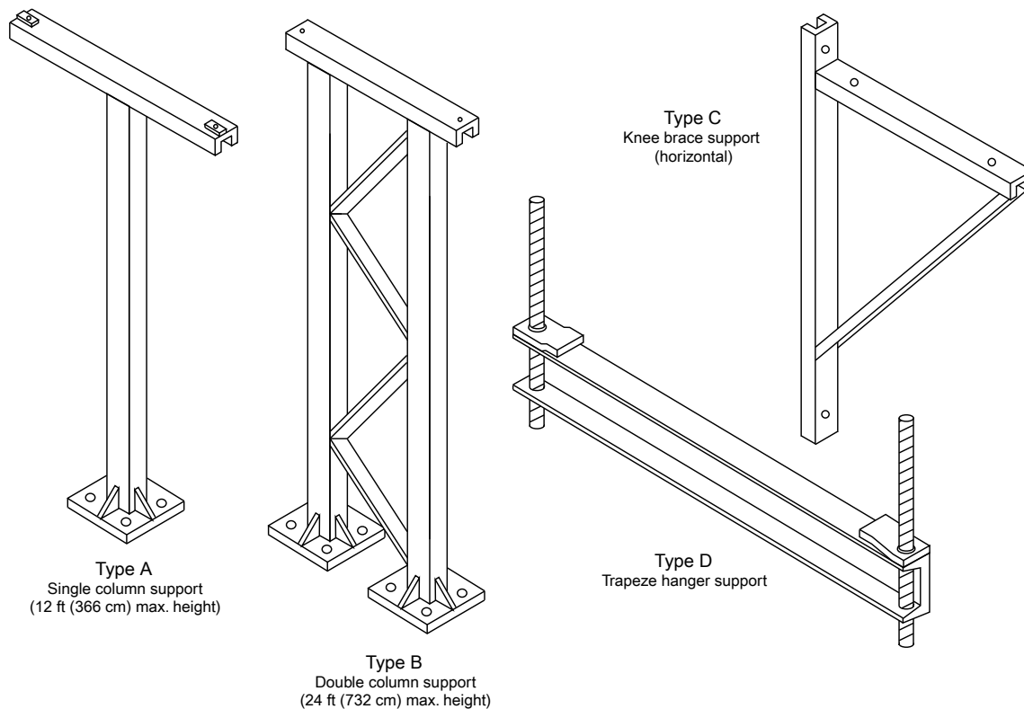
Figure 142 - Bus Supports
