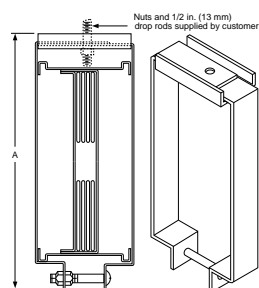
Figure 101 - Hanger (Horizontal Edgewise)
