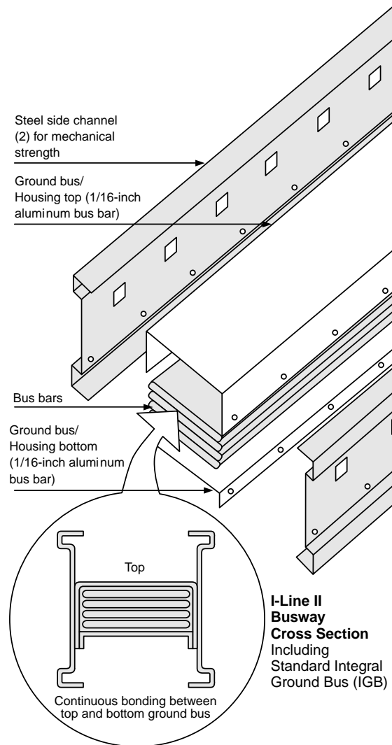
Figure 6 - I-Line II Busway Cross Section
