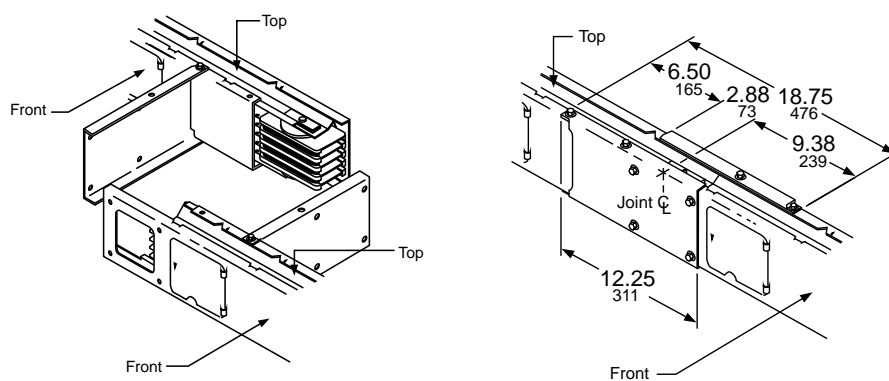
Figure 35 - Joint Detail
