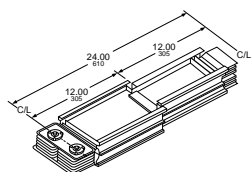
Figure 84 - Unfused Reducer (Indoor Only)
