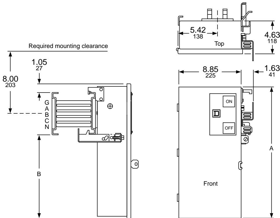
Figure 115 - Fusible Switch Plug-In Units — 30–100 A (Type “PQ”)
