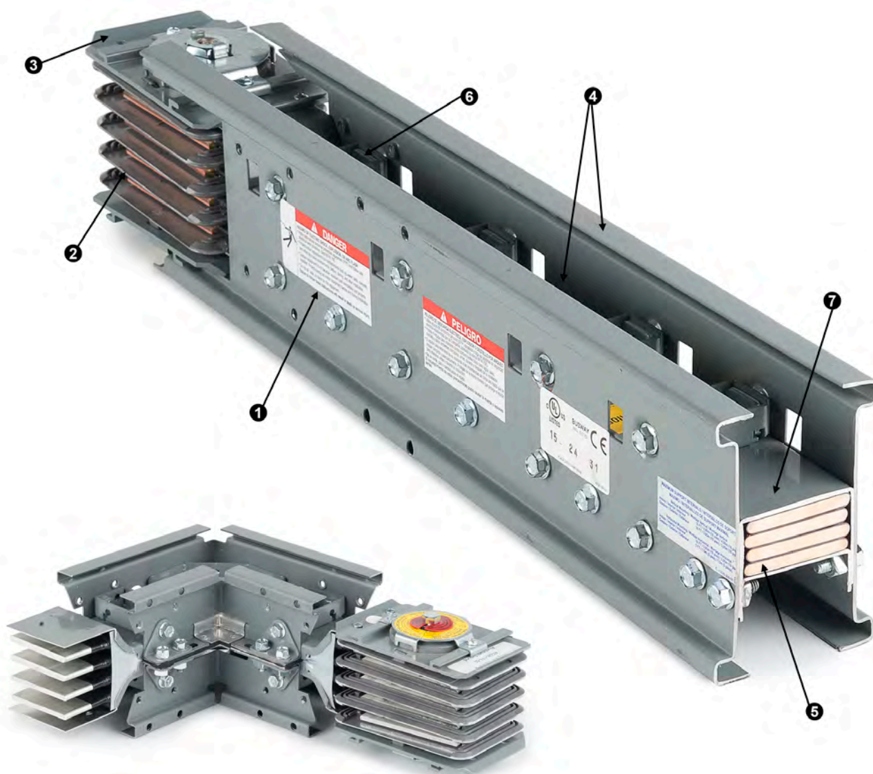
Figure 9 - Indoor Feeder Busway 800–5000 A
