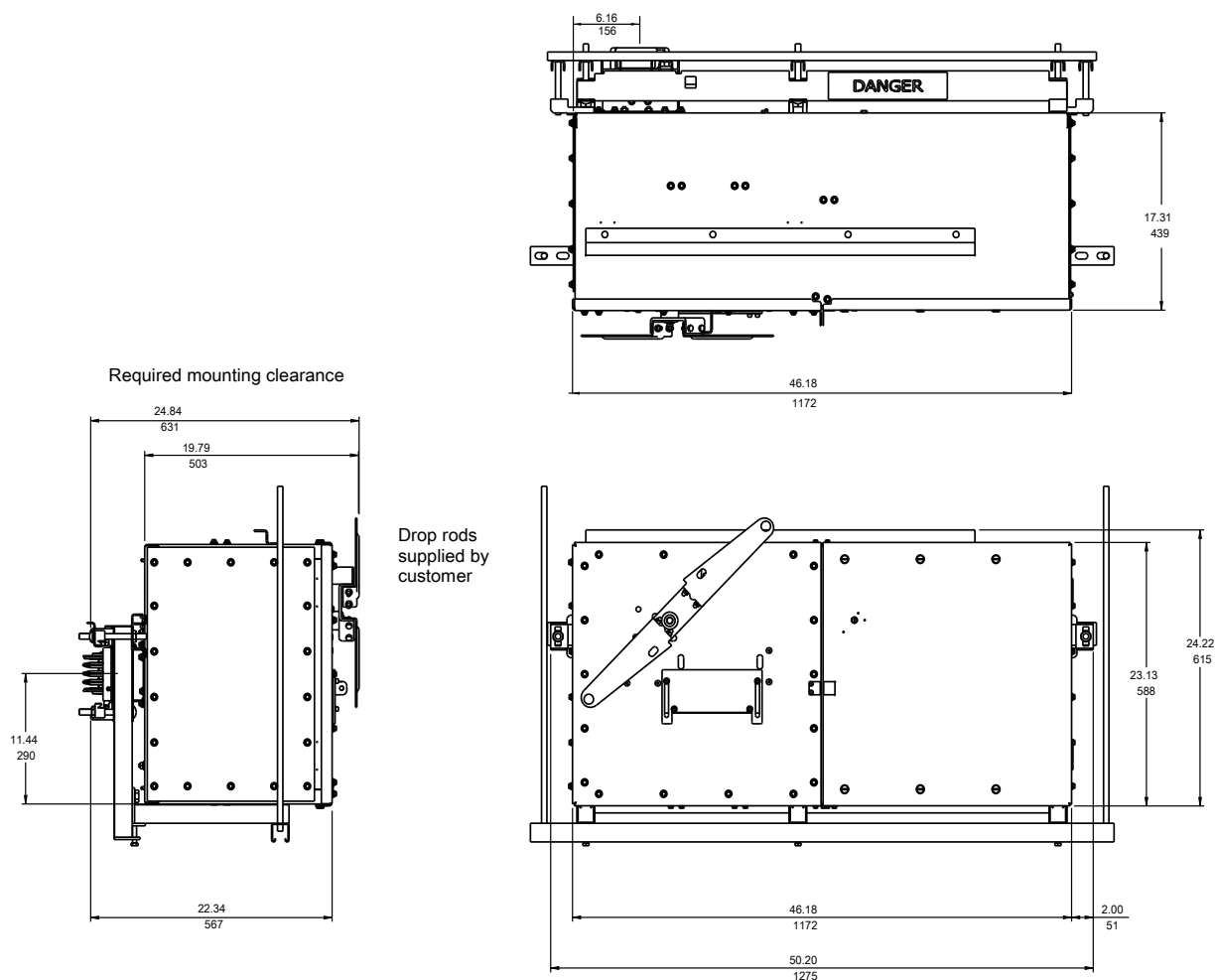
Figure 129 - Circuit Breaker Bolt-On Units (Horizontally Mounted)— 600–1600 A
