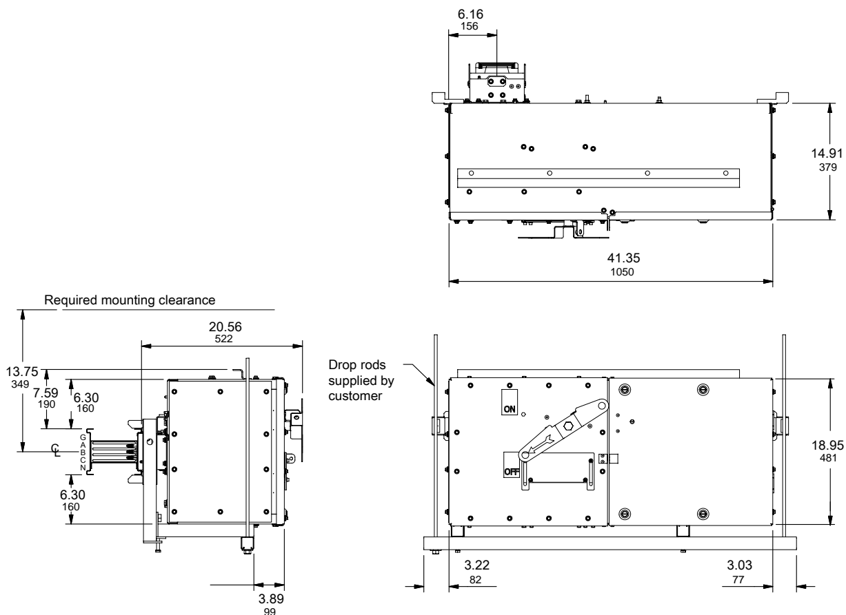
Figure 127 - Circuit Breaker Bolt-On Units (Horizontally Mounted)—250–1200 A
