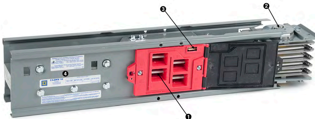
Figure 8 - Plug-In Busway 800–5000 A
