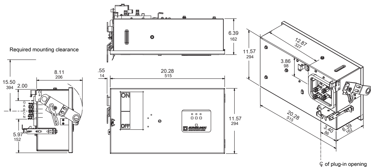
Figure 131 - Surge Protective Devices-Dimensions, Required Mounting Clearance
