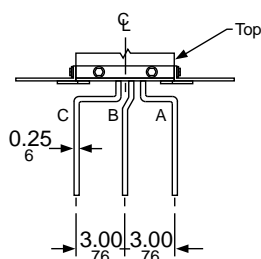
3-Pole
