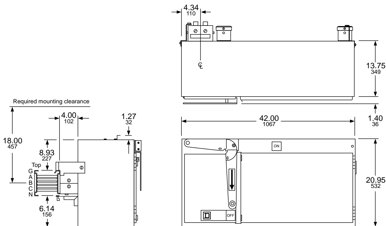
Figure 118 - Fusible Switch Plug-In Unit— 400 A and 600 A (Type “PBQ”)
