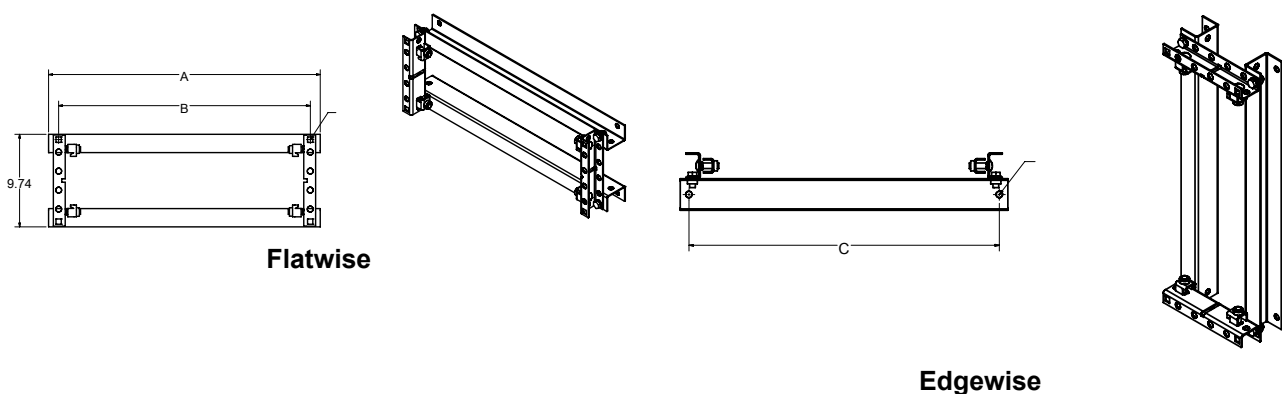
Figure 105 - Hanger (Horizontal Seismic)
