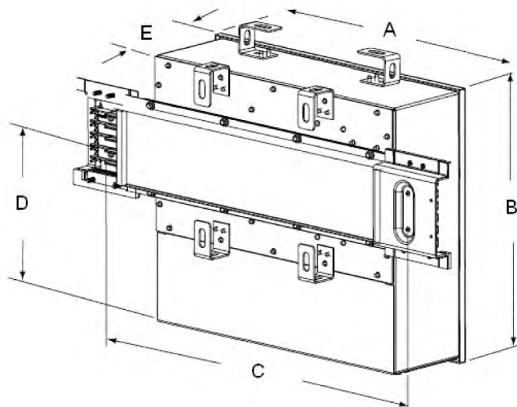
Figure 138 - Tap Box / Power Feed Unit
