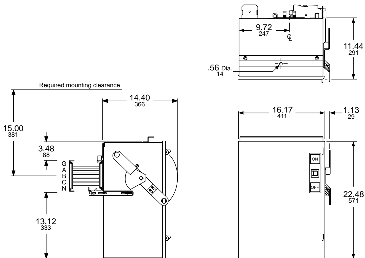
Figure 116 - Fusible Switch Plug-In Unit —200 A (Type “PQ”)
