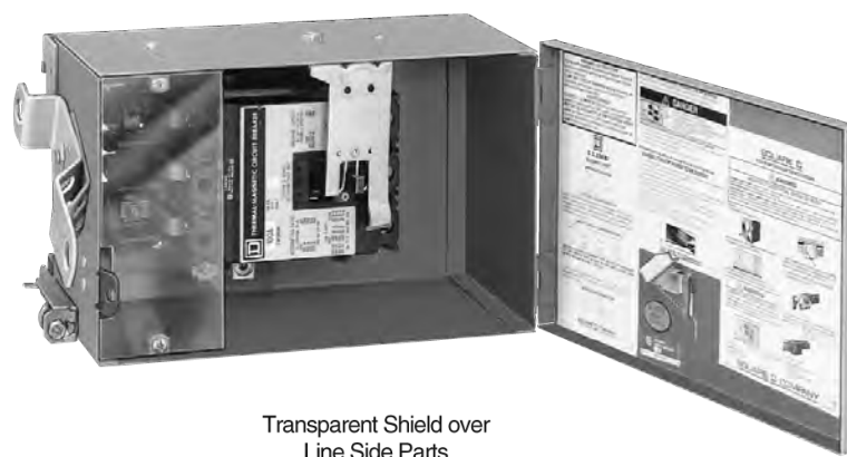
Figure 110 - Standard Molded Case Circuit Breaker
