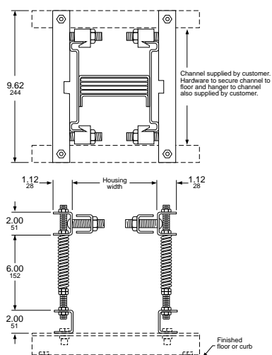
Figure 104 - Hanger (Vertical Spring)
