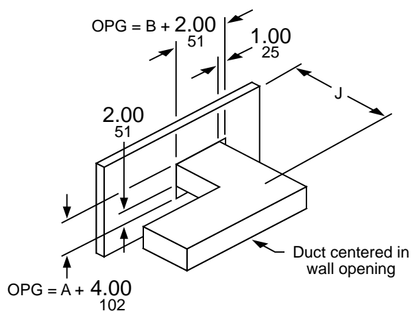
Wall Entrance
