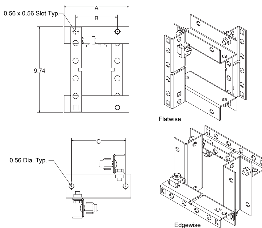
Figure 55 - Hanger (Horizontal Seismic) Dimensions
