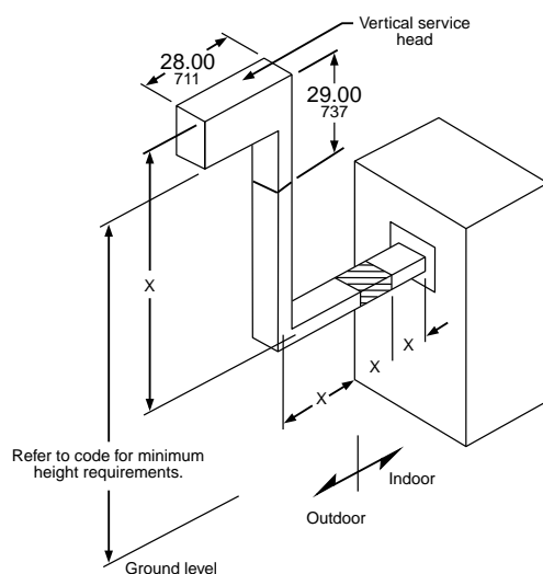
Figure 16 - Typical Vertical Service Head Application
