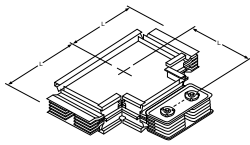
Figure 86 - Tees
