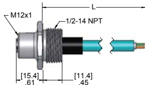
Female Receptacles
