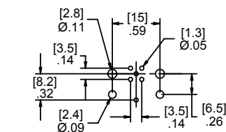
5 Pole Female Straight Layout
