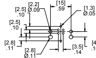
5 Pole Female Right Angle Layout
