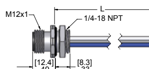
Male Receptacles
